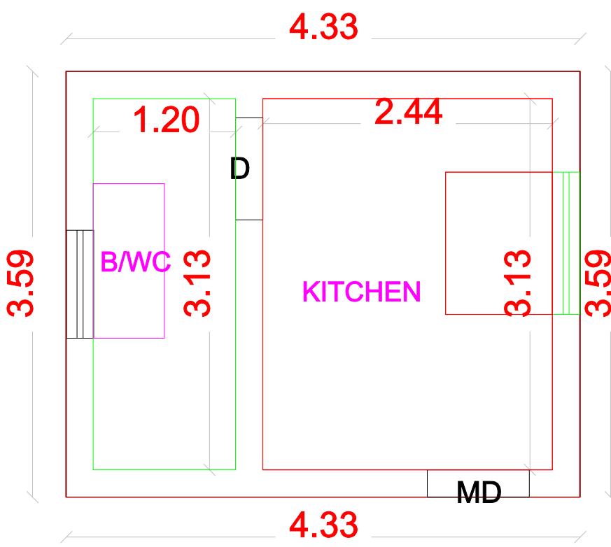
PLAN GROUND FLOOR ( PROPOSED )
