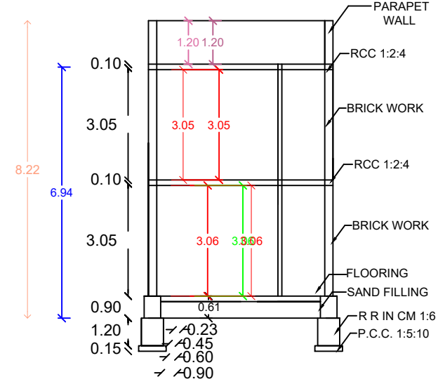
SECTION AB
