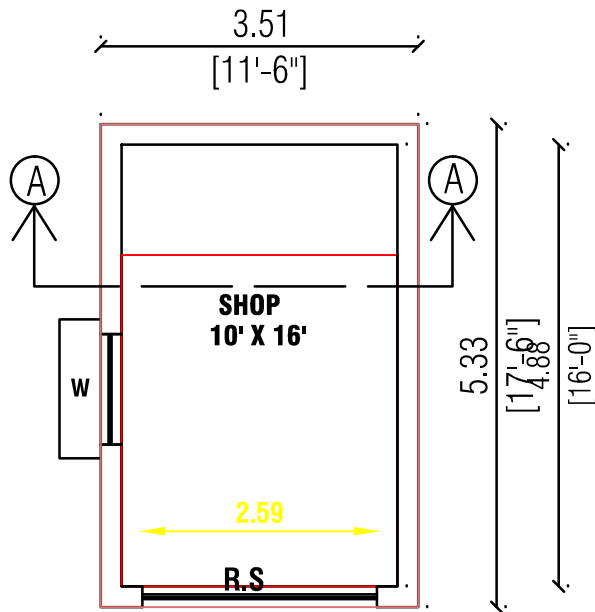
PLAN
