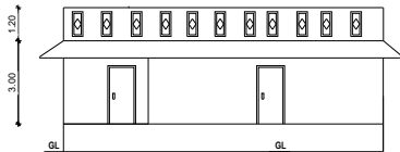
ELEVATION (PROPOSED)
