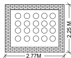
PLAN OF RWH
