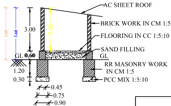
SECTION ON "BS"
