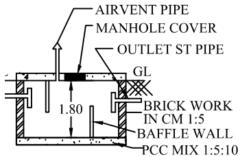
SECTION ON SEPTICTANK
