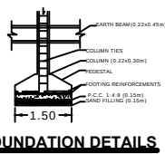
FOUNDATION DETAILS
