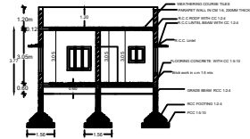
SECTION NON-AA
