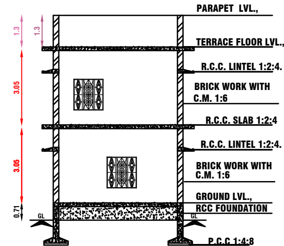
SECTION ON A-A & A'-A'
