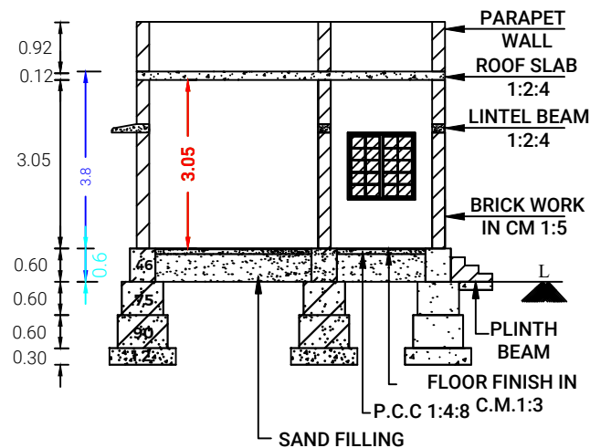
SECTION ON 'AA1'
