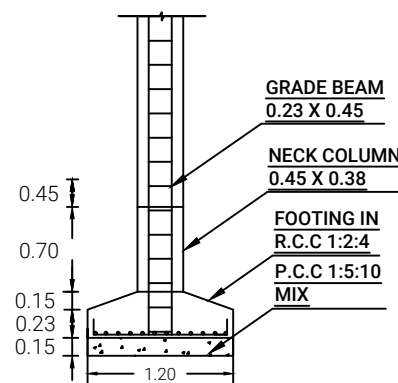
COLUMN DETAILS SCALE - 1:50
