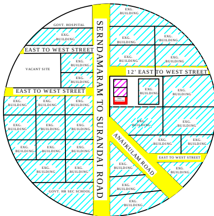
TOPO PLAN
