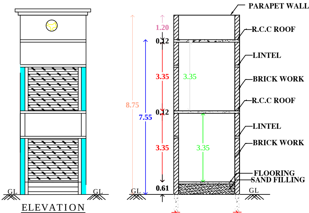
"SECTION "AB"
