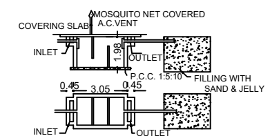
SEPTIC TANK & TRENCH U TRAP PROVISION
