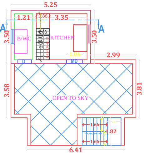
PLAN - FIRST FLOOR (PROPOSED)
