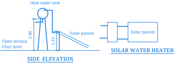
SIDE ELEVATION
