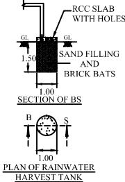
PLAN OF RAINWATER HARVEST TANK
