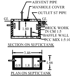
PLAN ON SEPTIC TANK
