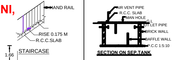
SECTION ON SEP.TANK
