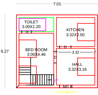
PROPOSED GF PLAN
