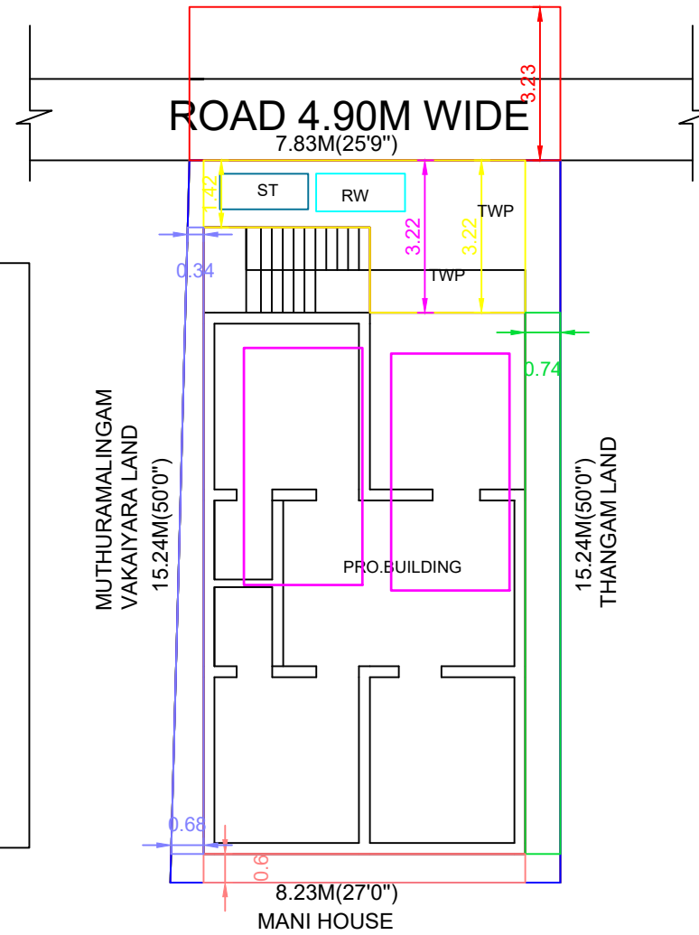
KEY PLAN
