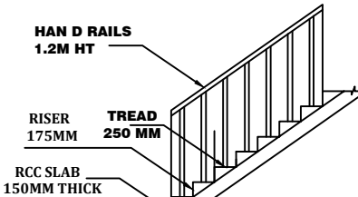
STAIRCASE DETAILS SCALE 1:50
