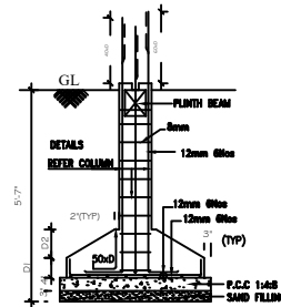
FOUNDATION DETAILS SCALE : 1:50.
