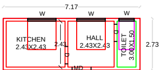
PROPOSED GF PLAN
