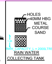
RAIN WATER COLLECTING TANK
