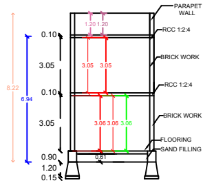
SECTION AB
