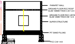
SECTION ON - AB
