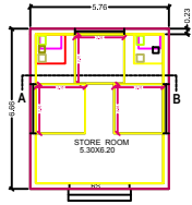
DETAILED GROUND FLOOR PLAN
