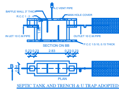
SEPTIC TANK AND TRENCH WITH U-TRAP ADOPTED
