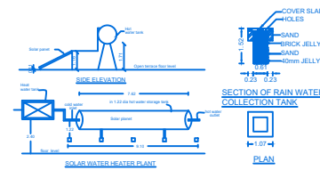
SOLAR WATER HEATER PLANT
