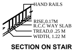
SECTION ON STAIR
