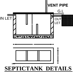
SEPTICTANK DETAILS
