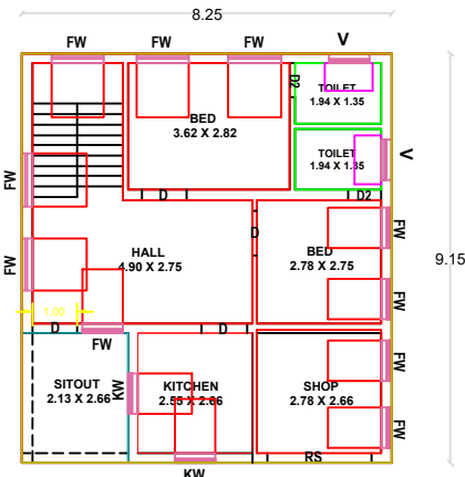
PLAN - GROUND FLOOR ( PROPOSED )
