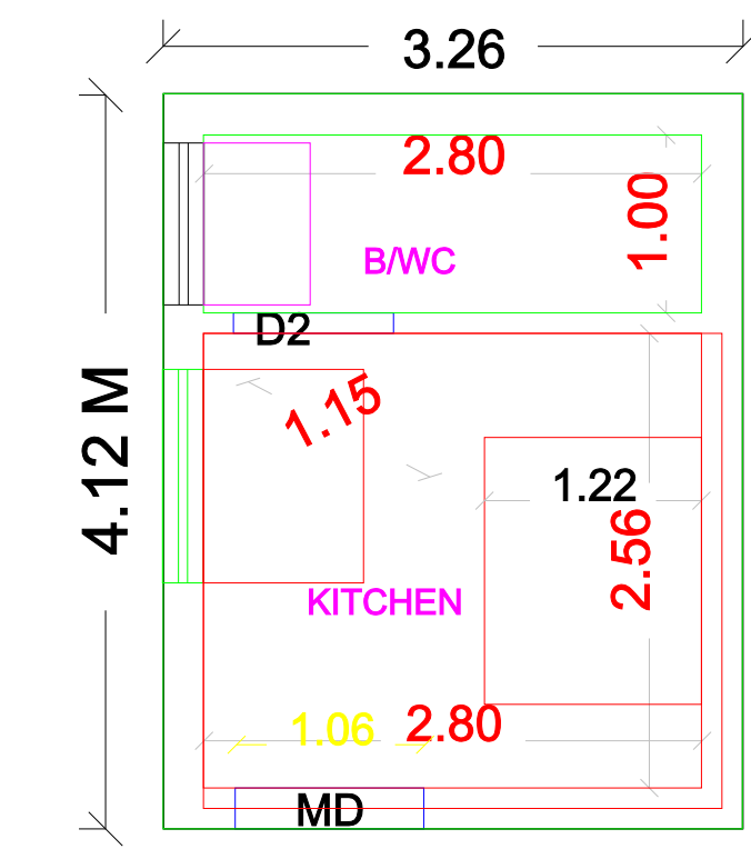
PLAN - GROUND FLOOR (PROPOSED)
