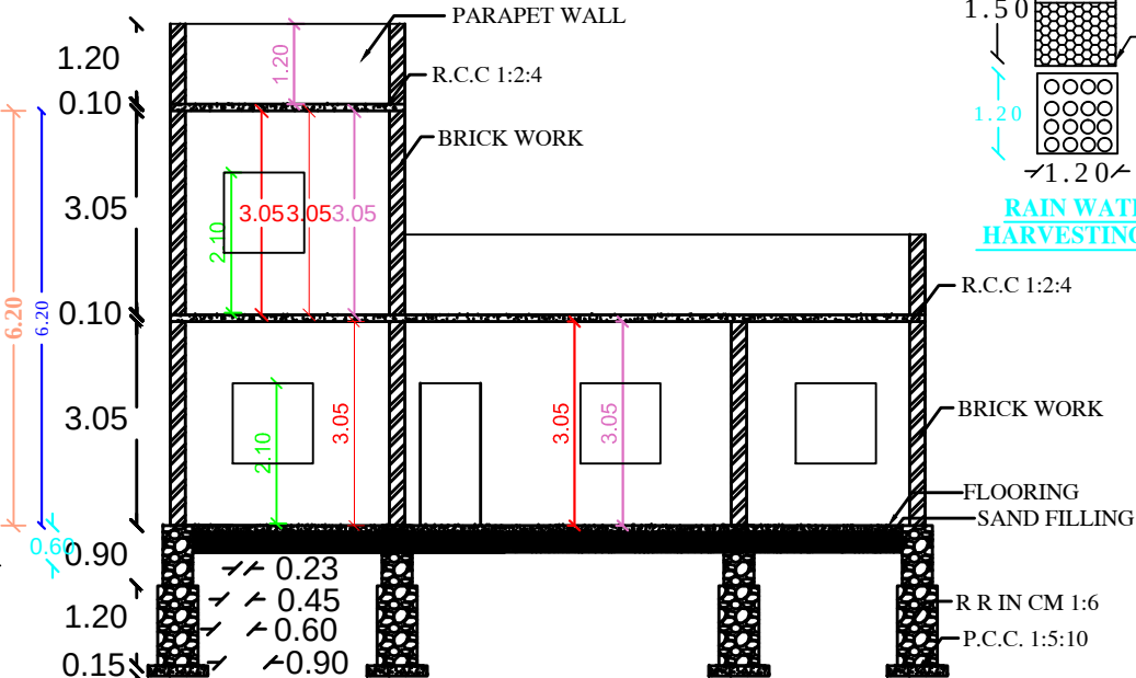
SECTION AB
