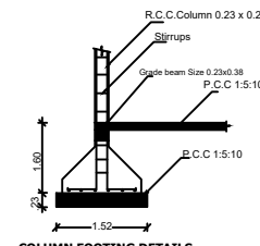
COLUMN FOOTING DETAILS
