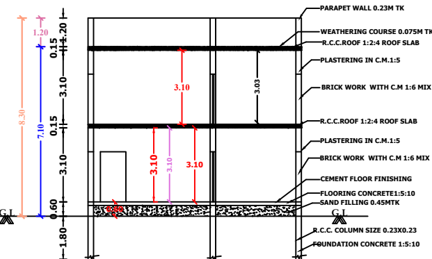
CROSS SECTION ON A-B
