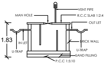
SECTION E,F SEPTIC TANK DETAIL
