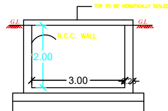
RWH SECTION
