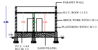
SECTION ON 'AA'
