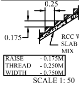
STAIR CASE DETAILS
