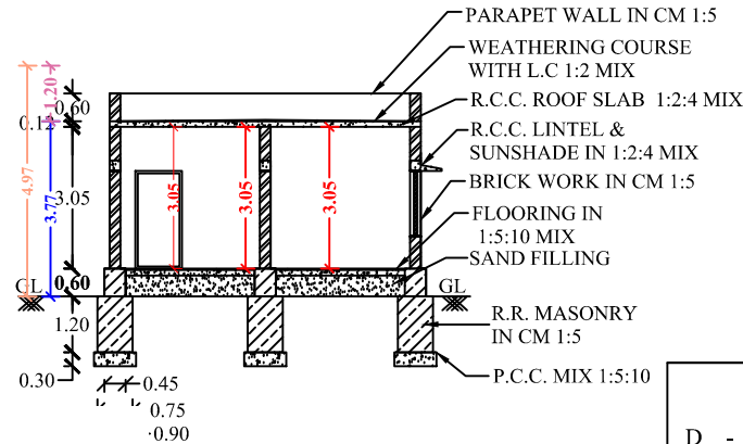
SECTION OF "AB"
