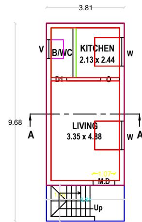
PLAN
