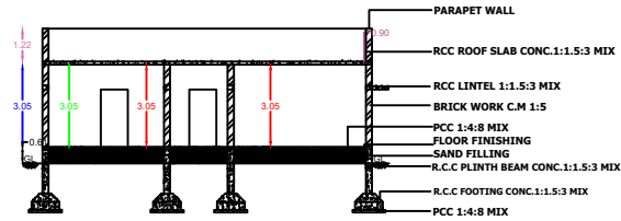
SECTION AB
