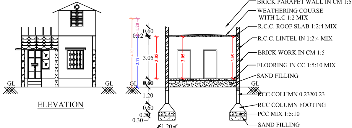
SECTION OF "AB"
