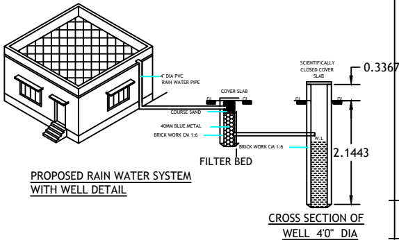
RWH SECTION
