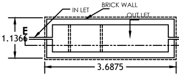
PLAN PLAN OF SEPTIC TANK
