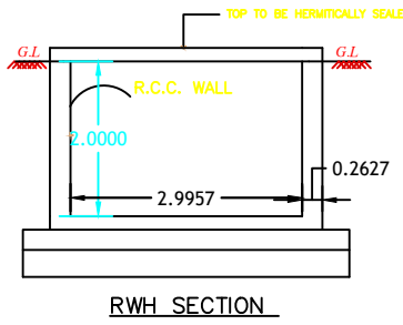
RWH SECTION
