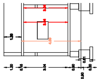
SECTION or
