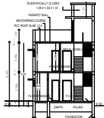
SECTION "A-B"
