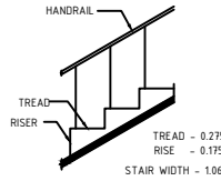
STAIRCASE DETAILS NTS
