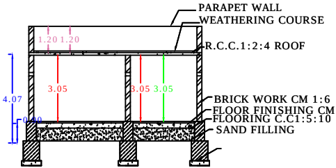
SECTION ON SV
