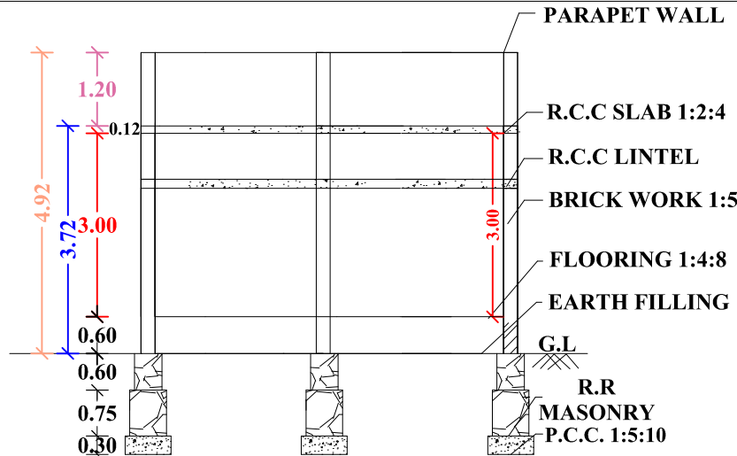
"SECTION "AB"
