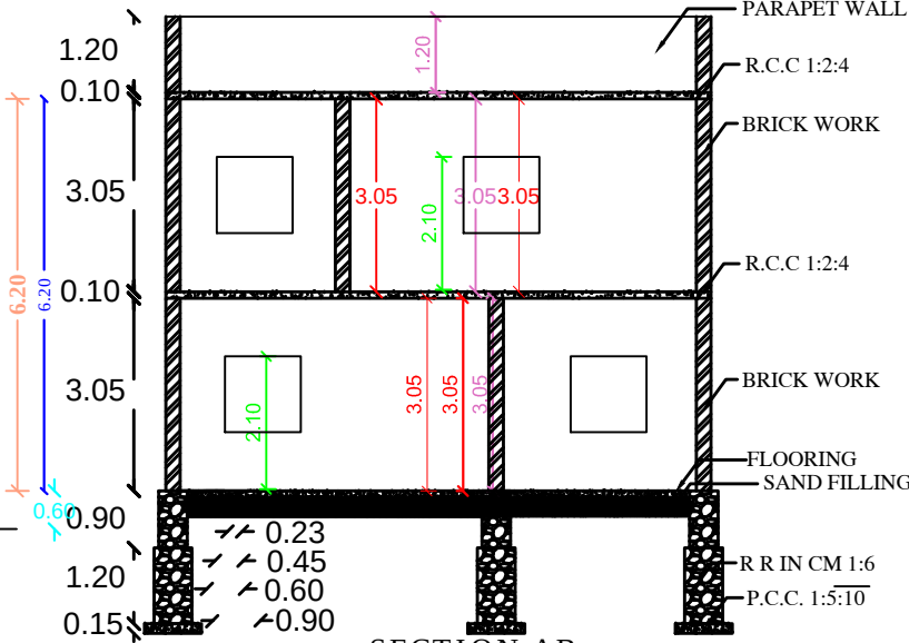
SECTION AB
