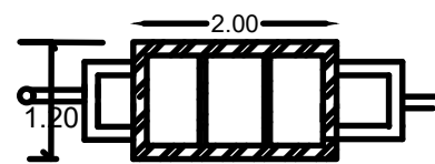
PLAN ON SEPTIC TANK
