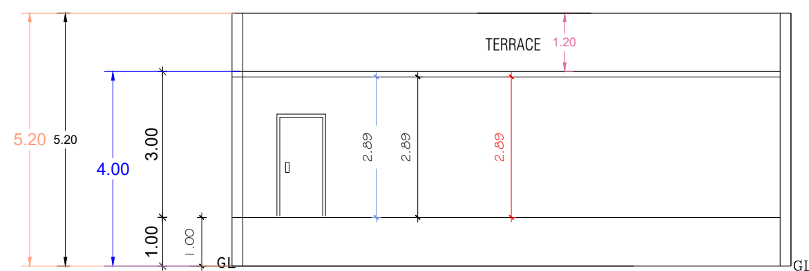
SECTION "A-A" (PROPOSED)
