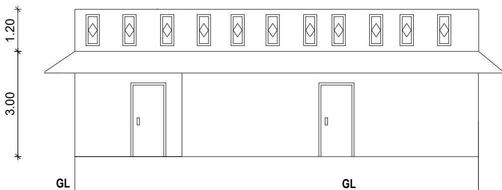
ELEVATION (PROPOSED)
