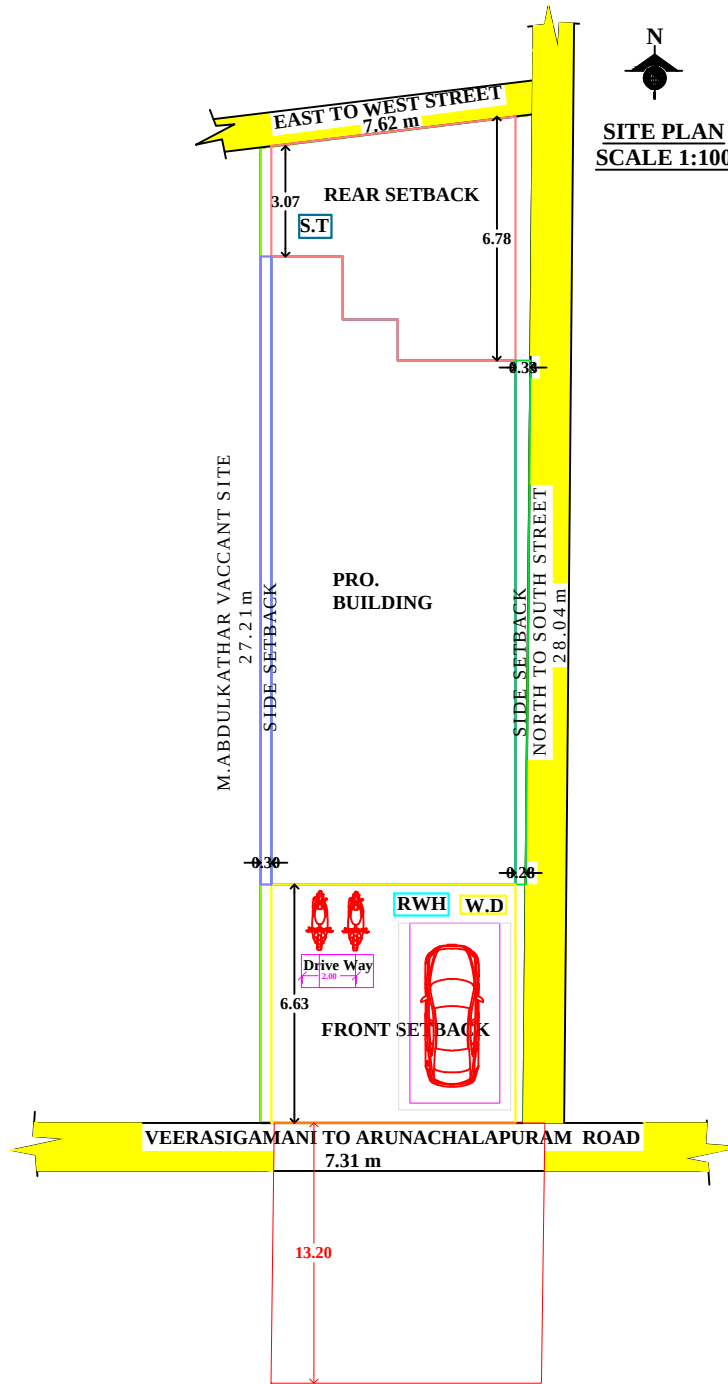
SITE PLAN
