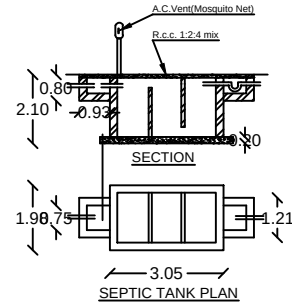
SEPTIC TANK PLAN
