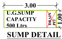
SUMP DETAIL
