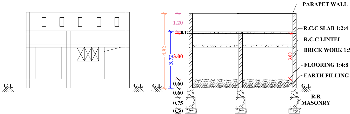
"FRONT ELEVATION"
