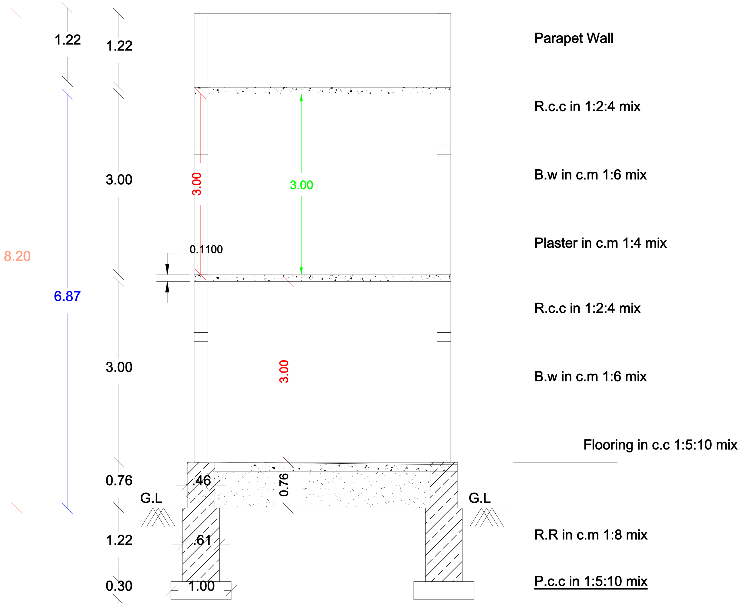
CROSS SECTION
