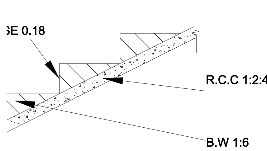
STAIRCASE DETAILS
