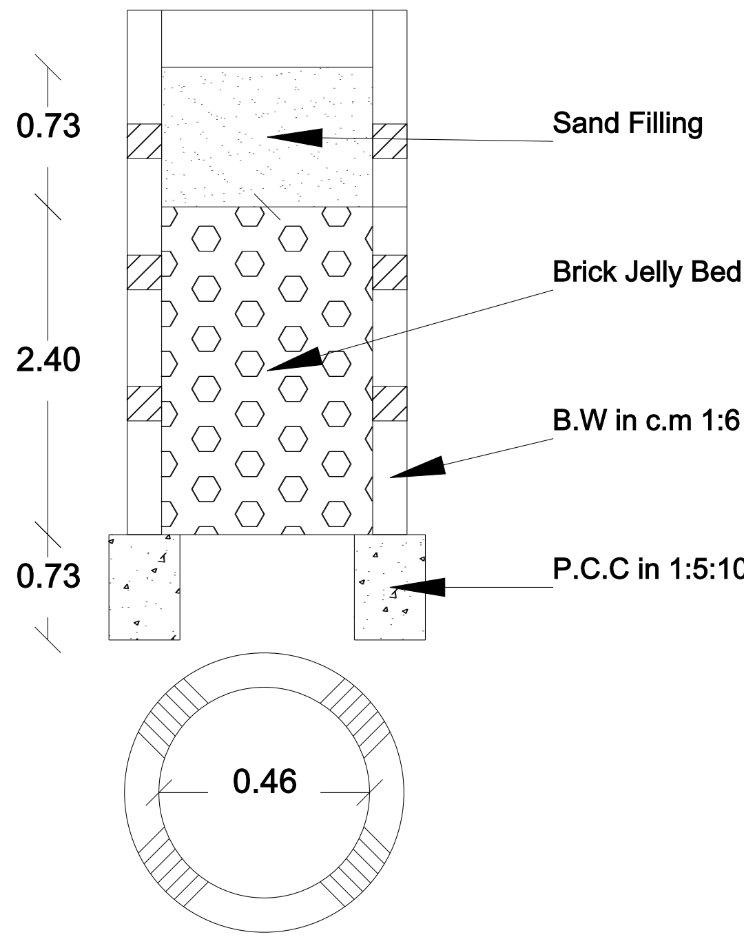
RAIN WATER HARVESTING
