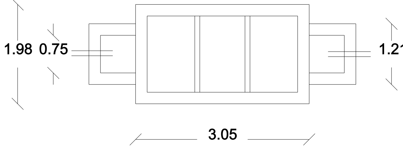
SEPTIC TANK PLAN
