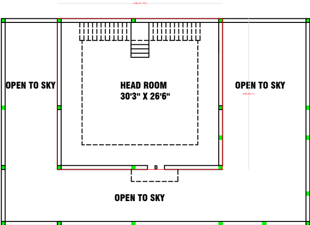
HEAD ROOM PLAN
