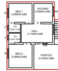
EXS BUILDING-3 GROUND FLOOR PLAN
