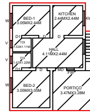
EXS BUILDING-3 GROUND FLOOR PLAN
