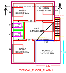
PRO BUILDING-5 GROUND FLOOR PLAN
