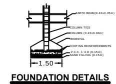
FOUNDATION DETAILS
