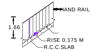
STAIRCASE
