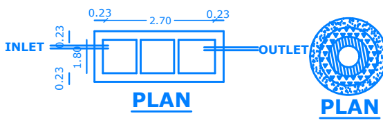
SEPTICTANK DETAILS LEACH WELL DETAILS
